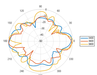
Elevation 2: 3400 – 3800 MHz
