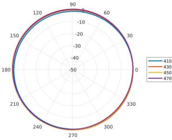
Azimuth: 410 – 470 MHz
