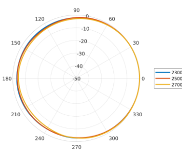
Azimuth: 2300 – 2700 MHz
