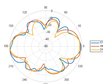
Elevation 2: 1710 – 2100 MHz
