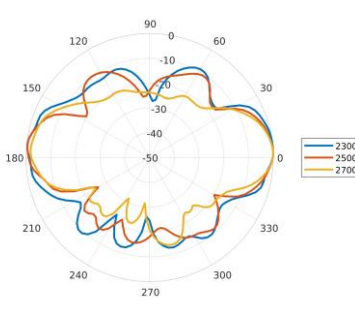
Elevation 2: 2300 – 2700 MHz
