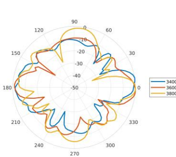
Elevation 1: 3400 – 3800 MHz
