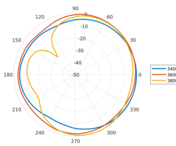
Azimuth: 3400 – 3800 MHz
