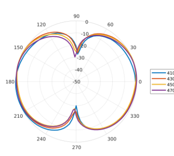
Elevation 2: 410 – 470 MHz
