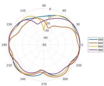
Elevation 1: 690 – 960 MHz
