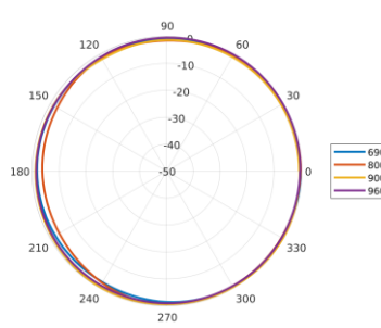
Azimuth: 690 – 960 MHz
