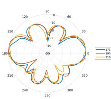
Elevation 2: 1710 – 2100 MHz
