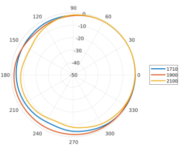
Azimuth: 1710 – 2100 MHz
