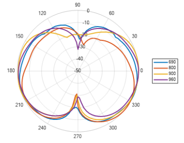
Elevation 2: 690 – 960 MHz
