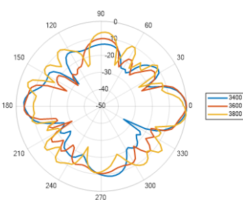
Elevation 1: 3400 – 3800 MHz
