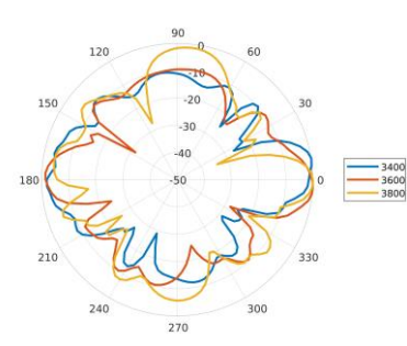
Elevation 2: 3400 – 3800 MHz
