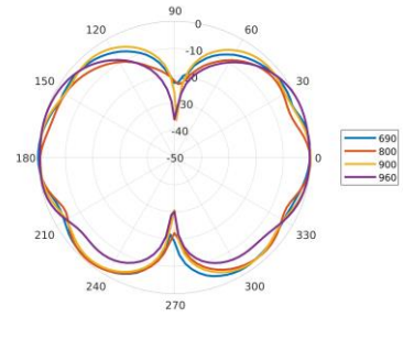
Elevation 2: 690 – 960 MHz
